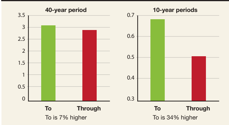
FIGURE 4: REWARD-TO-RISK RATIOS, 1926–2008
