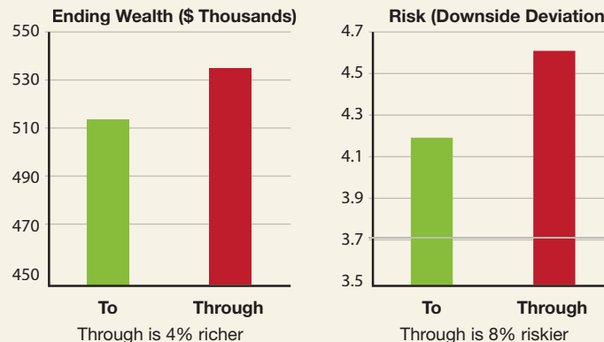
FIGURE 3: TO VERSUS THROUGH GLIDE PATH COMPARISONS, 1926–2008 (74 10-YEAR PERIODS)
